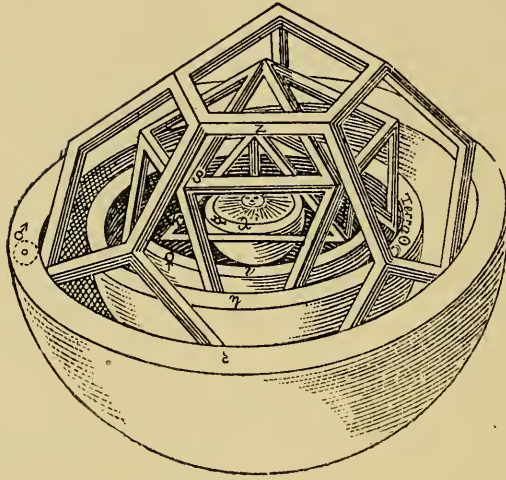
Kepler's system of regular solids.
