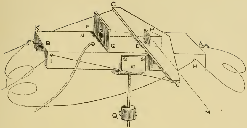
Astronomer made by Sir J. Herschel to compare the light of certain stars by the intervention of the moon.
