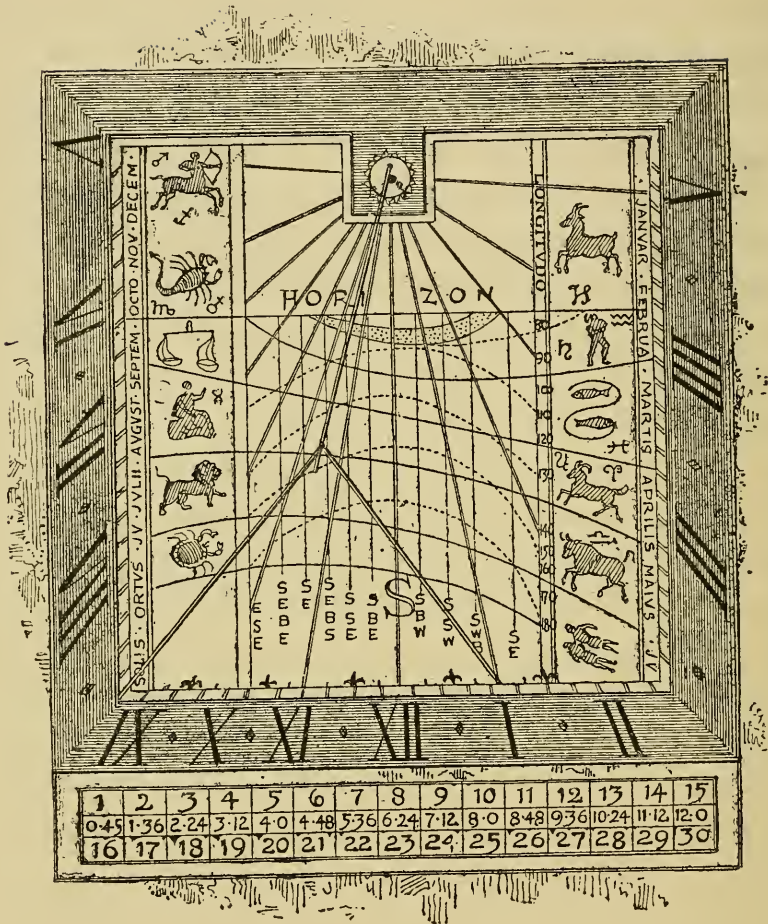
Sir Isaac Newton's Sun-dial.
